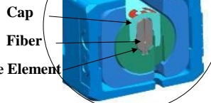
Cross-sectional view of actuated splice
