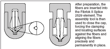
Cross-sectional view of open and actuated Fibrlok II Splice 2529
