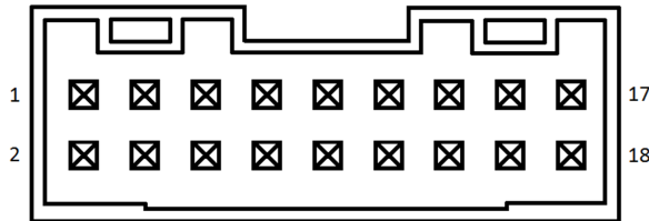
Figure 5 PLC Connector (looking at UV Head).
