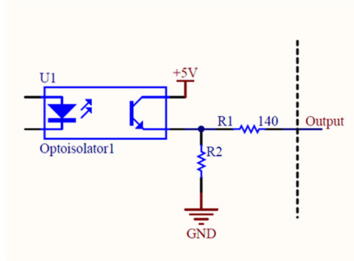
Figure 6 PLC digital output equivalent circuit
