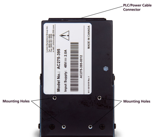
Figure 3 UV LED Head (back)
