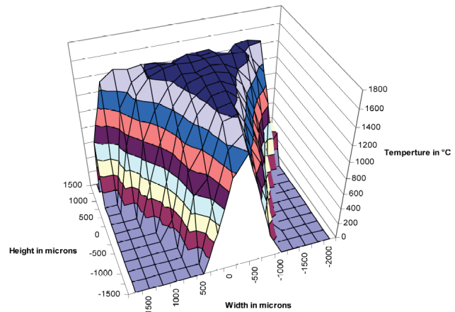
Figure 3: Three phase arc thermal profile A
